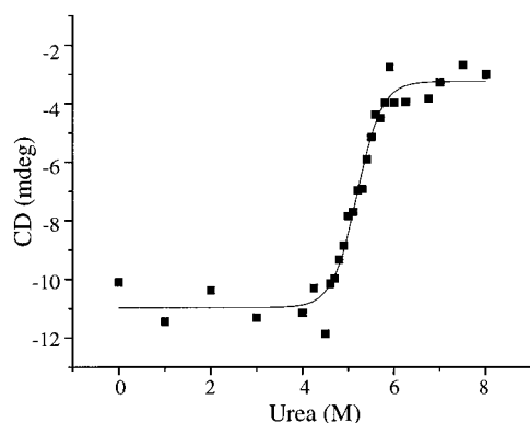
FIGURE 6: Solvent denaturation of E2 cd under reducing conditions. Individual samples of enzyme were denatured in a series of concentrations of urea in 50 mM KP i , 100 mM KCl, 2.5 mM DTT, pH 6.8, at 30 °C. The C_m is 5.2 M; the m -value is 2.2 kcal/(mol•M); the \Delta G_u is 11.2 kcal/mol.
